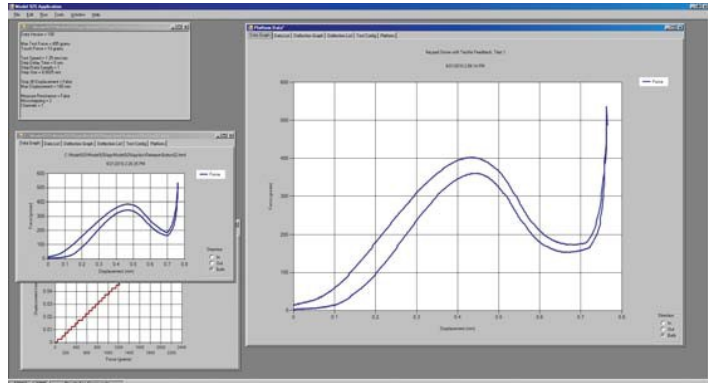
Force-Distance Graph
